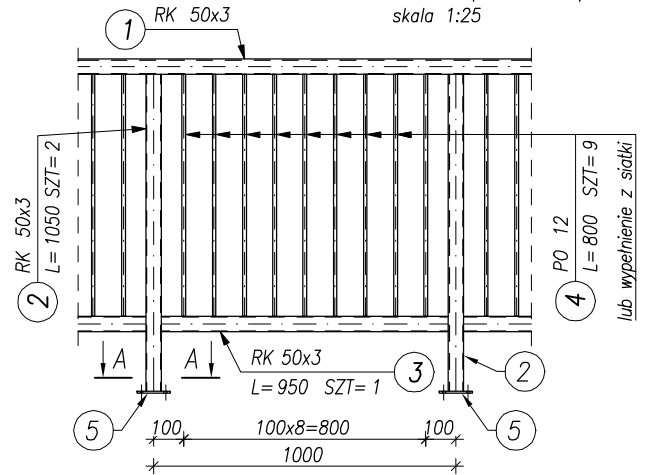
BR-1 barierka (50.6 mb) skala 1:25
